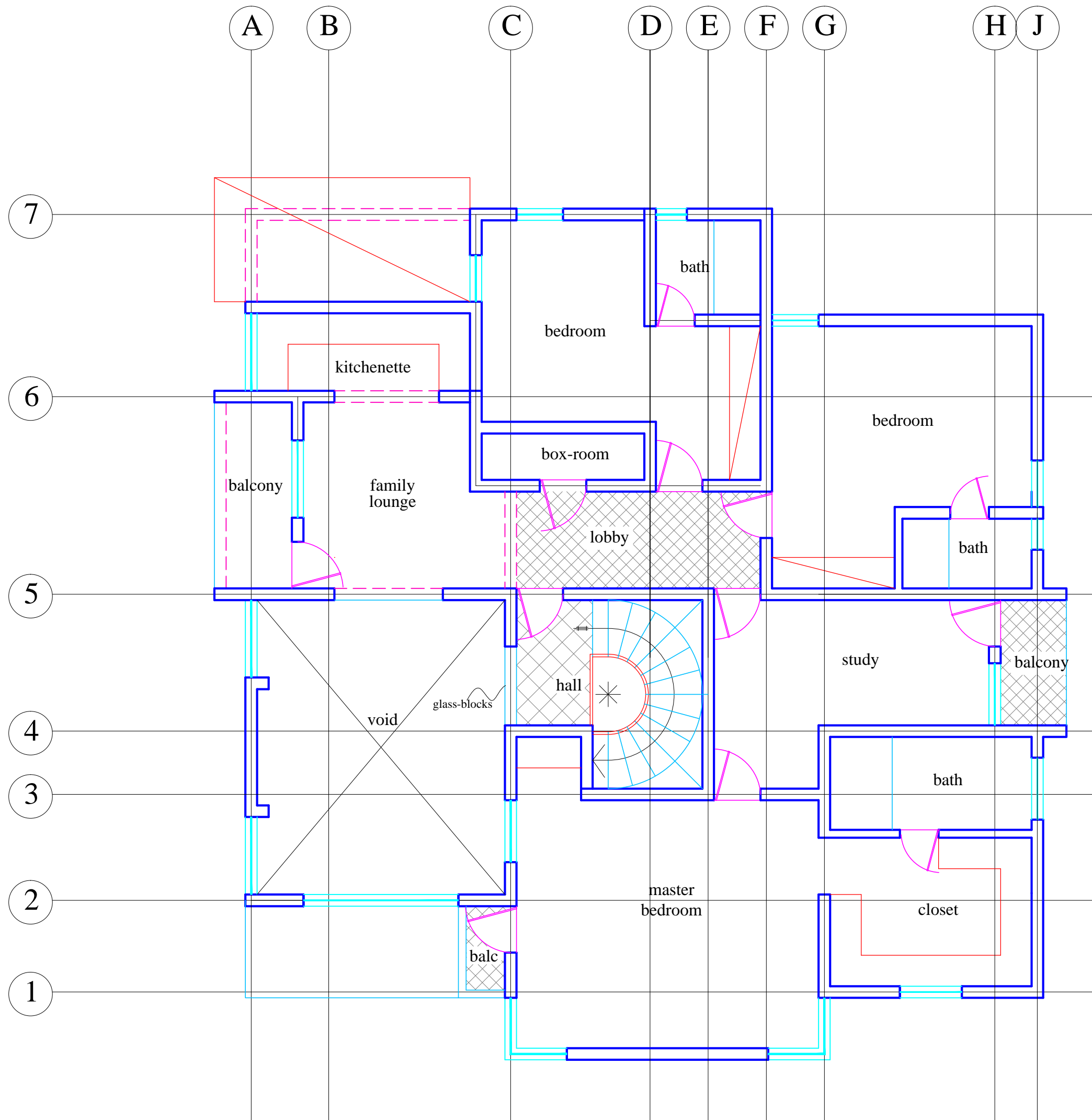
UPPER FLOOR PLAN
